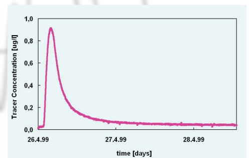
Breakthrough-curve of Eosin in groundwater
